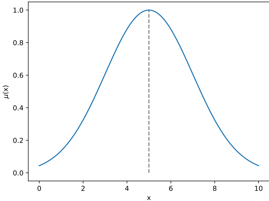
Gaussian(mu=5, sigma=2)
