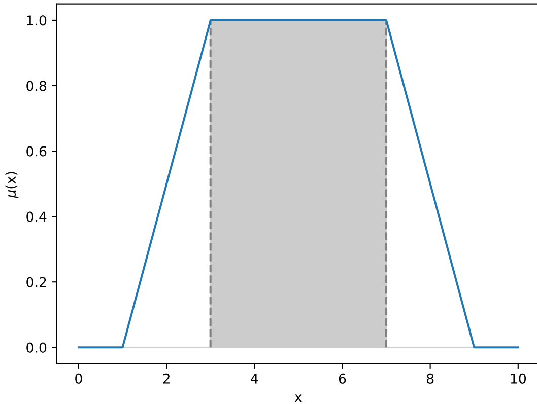
Trapezoid(a=1, b=3, c=7, d=9)
